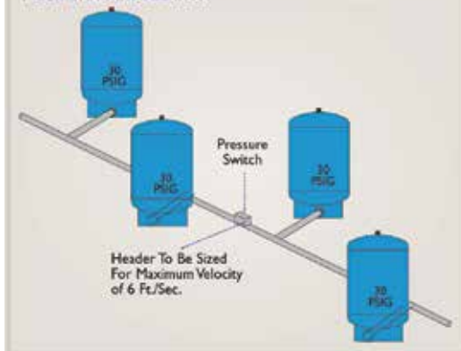
MULTI-TANK INSTALLATION
